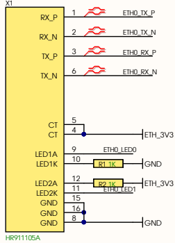
10/100 Mb Ethernet
