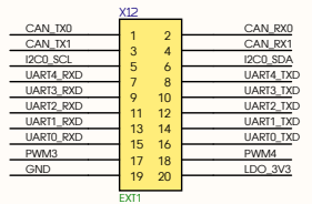
EXT interfaces
