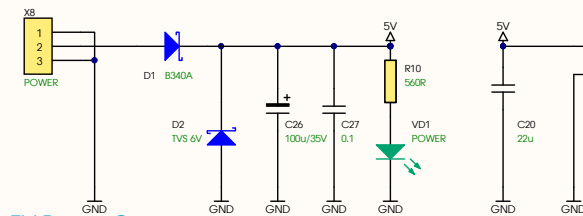
5V Power Connector
